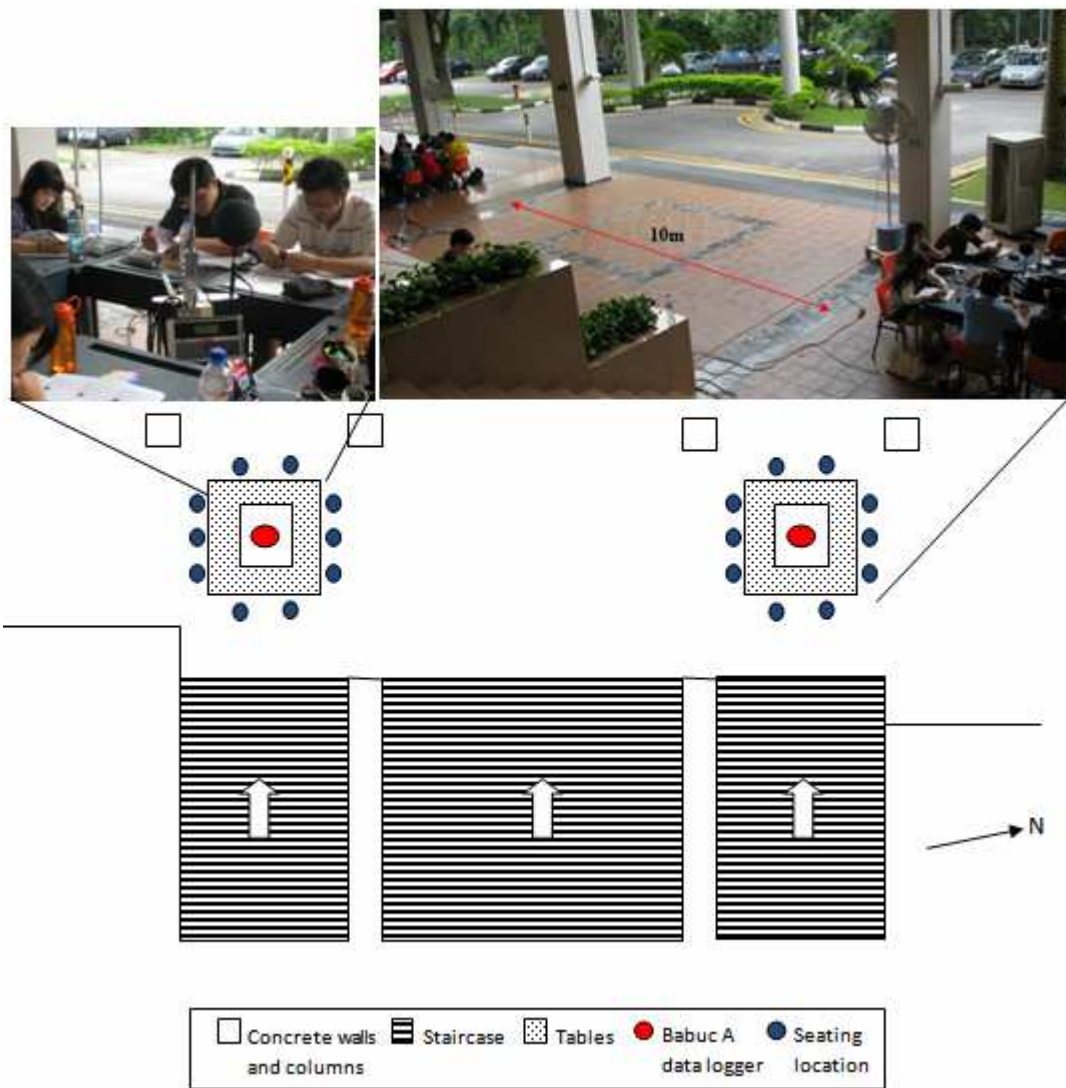
Figure 1. Experimental setup at NUS
